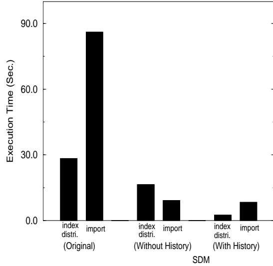
Figure 5. Execution time for partitioning indices and data in FUN3D
