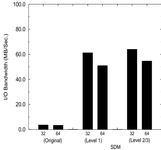
Figure 7. I/O bandwidth for RT
