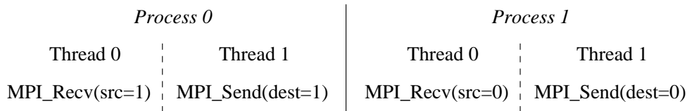
Figure 1: An implementation must ensure that this example never deadlocks for any ordering of thread execution.
