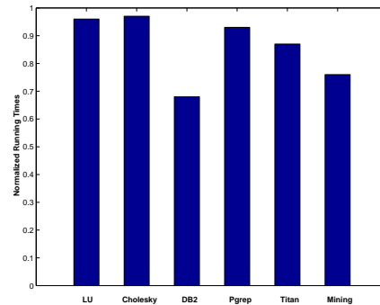
Figure 5. Benefits of runtime bypassing on application traces.
