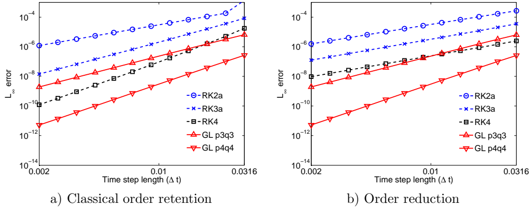
FIG. 7.2. Order analysis for the classical SSP RK methods of orders two and three (blue), the fourth order RK method, and SSP GL methods GLp3q3 (C.42) and GLp4q4 (D.51) (red). The GL methods preserve their corresponding orders, whereas the classical RK methods suffer from order reduction.
