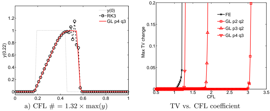
FIG. 7.3. (a) Solution of the Burgers' equation using the third-order RK method ( s = 3 , C = 1 ) and fourth order GLp4q3s3k3 (D.43) ( C = 1.07 ). In (b) we show the maximum change of the solution TV with forward Euler (FE) C = 1 and GL methods of orders two (6.1) C = 2.57 , three (C.24) C = 1.65 , and four (D.43) C = 1.07 . The theoretical results are verified.
