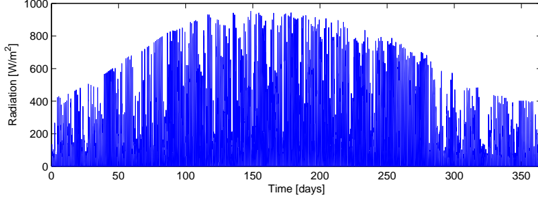
Figure 5: Total solar radiation in Chicago, IL, 2004.
