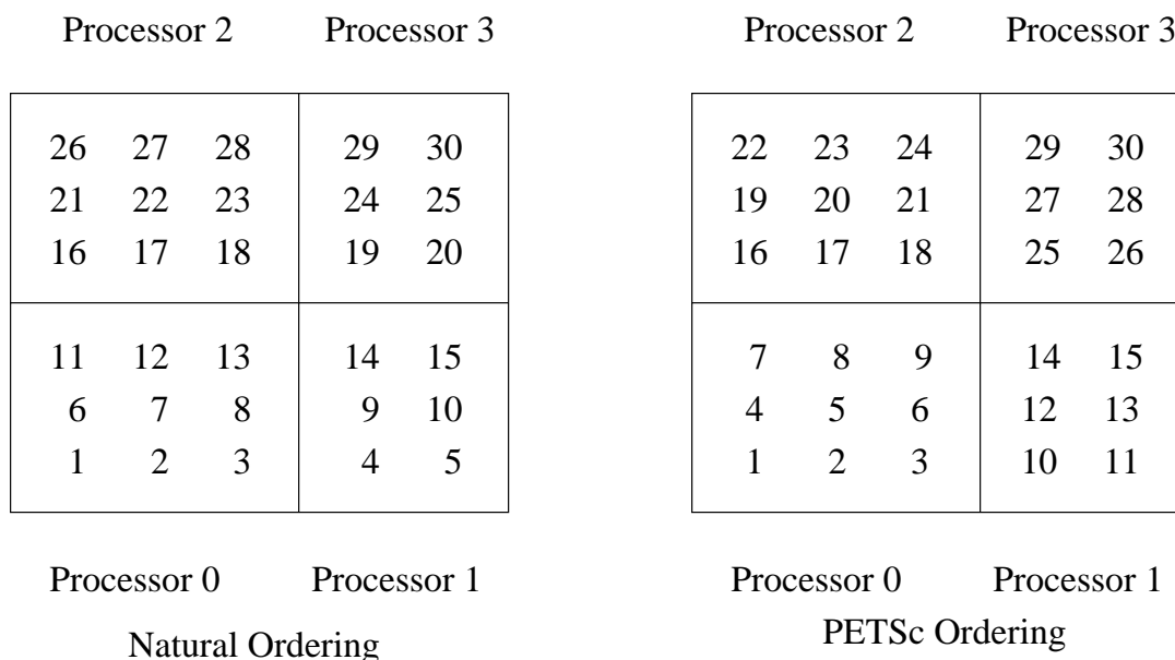
Figure 9: Natural Ordering and PETSc Ordering for a 2D Distributed Array (Four Processes)
