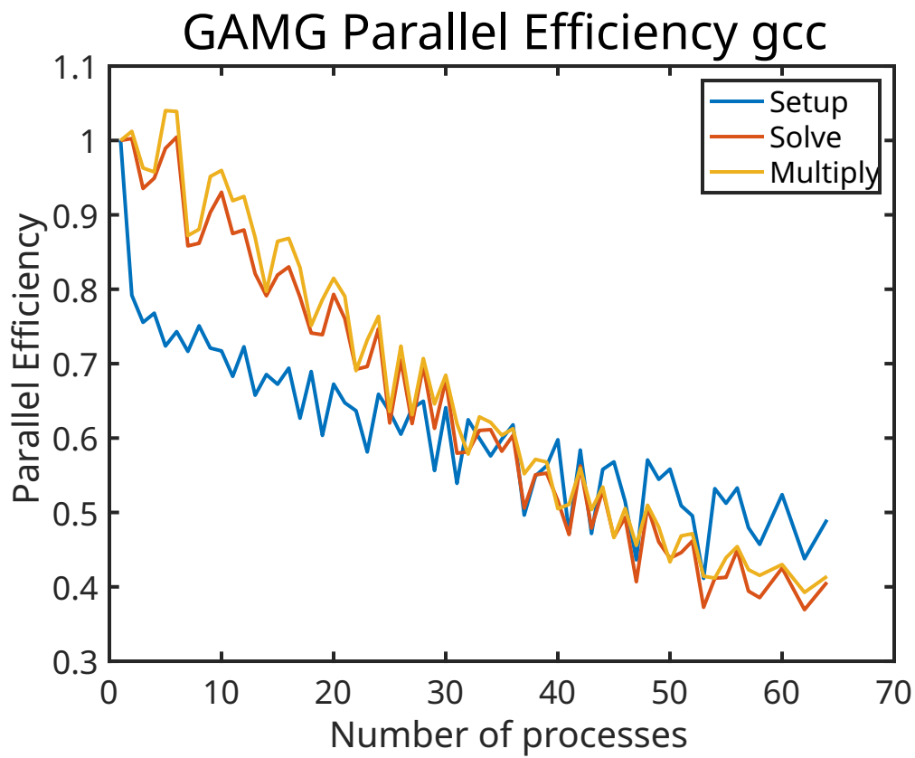
Fig. 4.12: GAMG parallel efficiency
