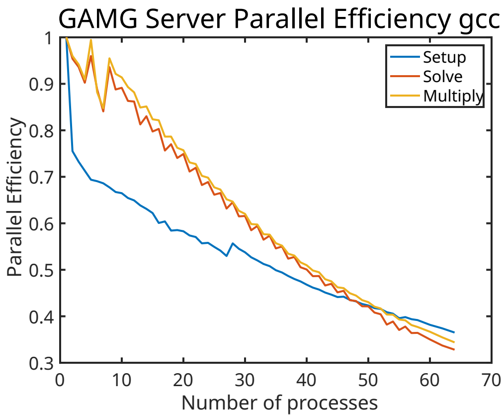
Fig. 4.15: GAMG server parallel efficiency
