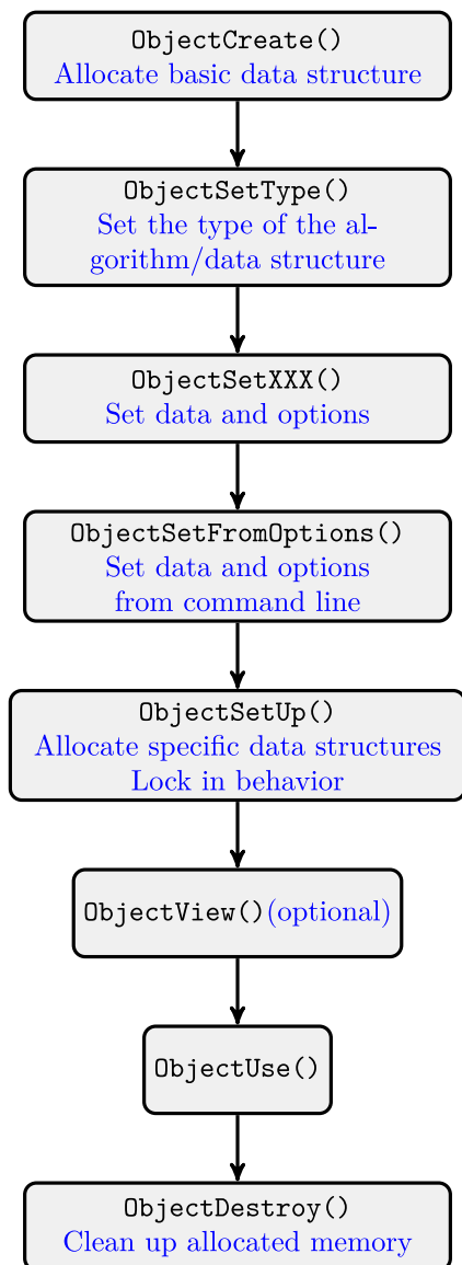
Fig. 1.2: Sample lifetime of a PETSc object
