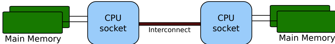
Fig. 3.2: Schematic of a two-socket NUMA system. Processes should be spread across both CPUs to obtain full bandwidth.
